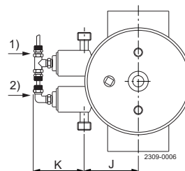
1) CIP valve
